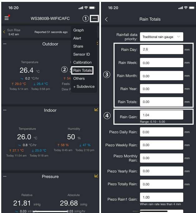
Figure 45: Rainfall Calibration
